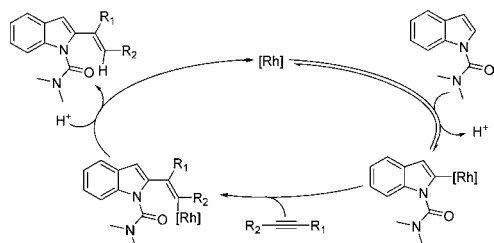
Figure 1. Proposed catalytic cycle.
